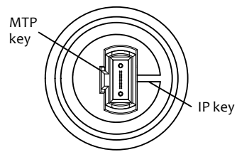
VIEW TO CONNECTOR MPO FEMALE
