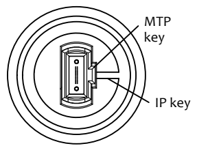
VIEW TO CONNECTOR MPO MALE
