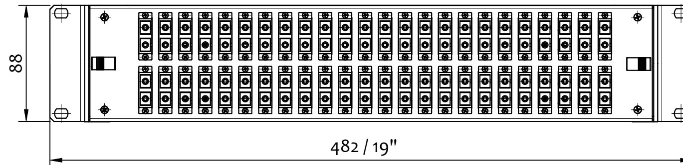
48x SC DX (FRONT VIEW)
