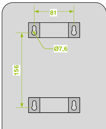
Mounting dimensions
