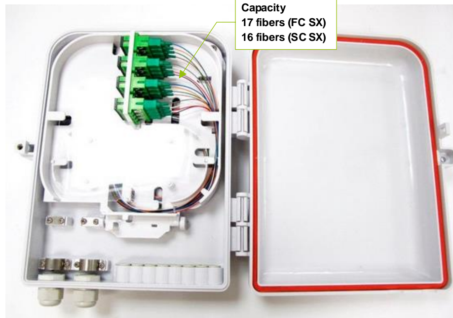
Inside view
